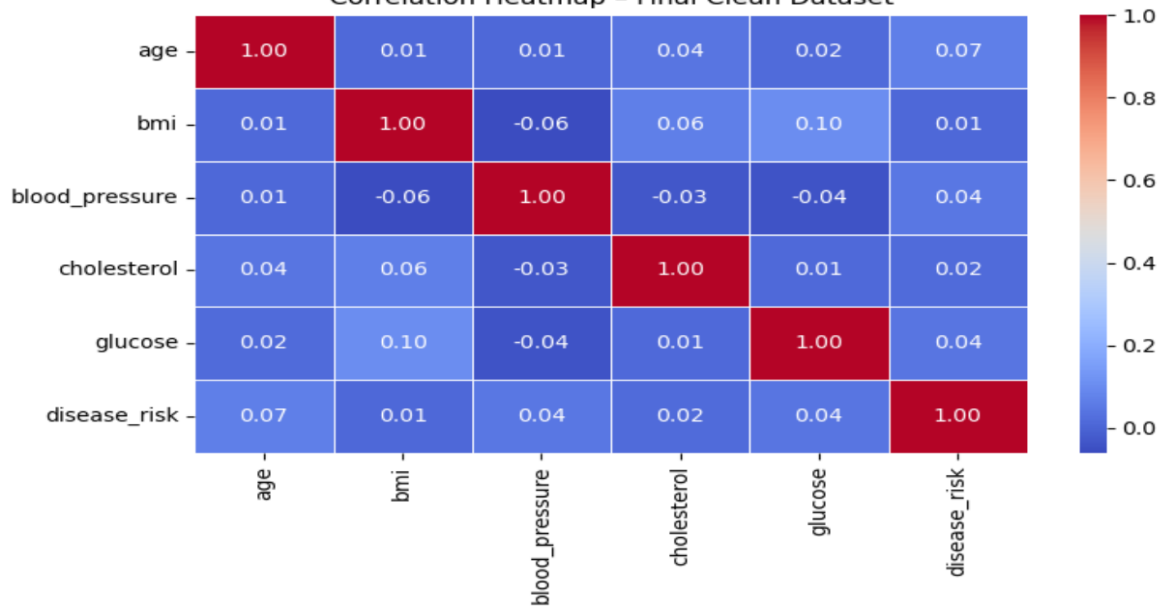
Correlation Heatmap - Final Clean Dataset
