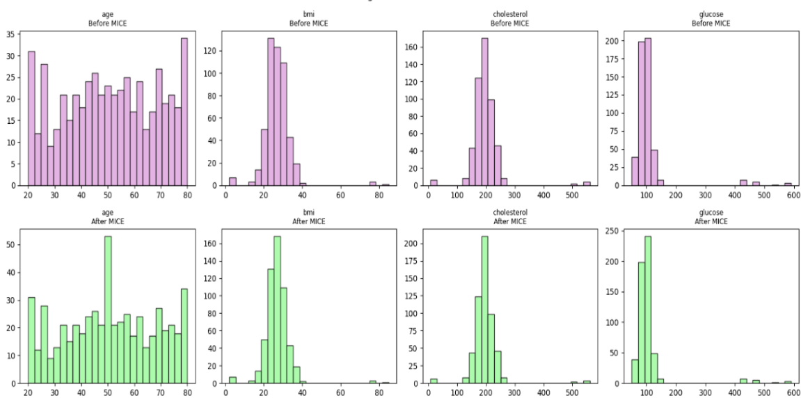
MICE Algorithm - Before vs After
