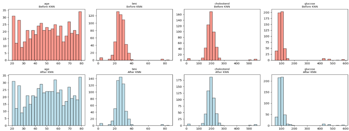
KNN Imputer - Before vs After
